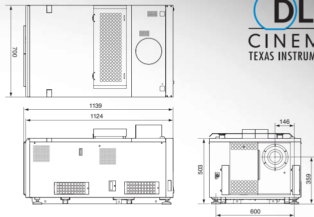
■ External Diagram (NC3240S)
