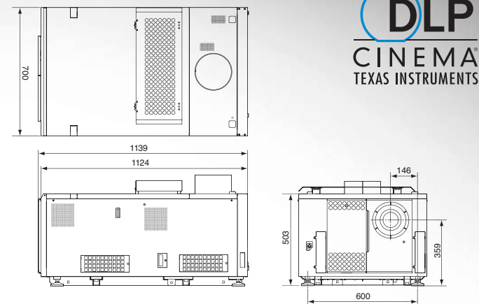
■ External Diagram (NC3200S)
